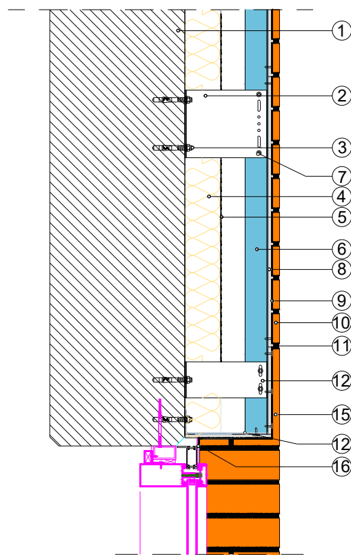
WINDOW TOP CONNECTION SECTION
