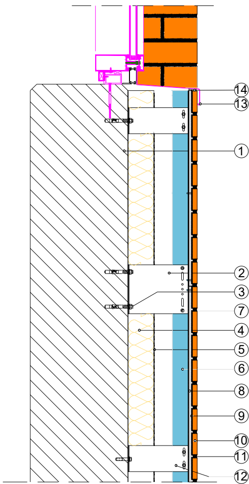
WINDOW BOTTOM CONNECTION SECTION
