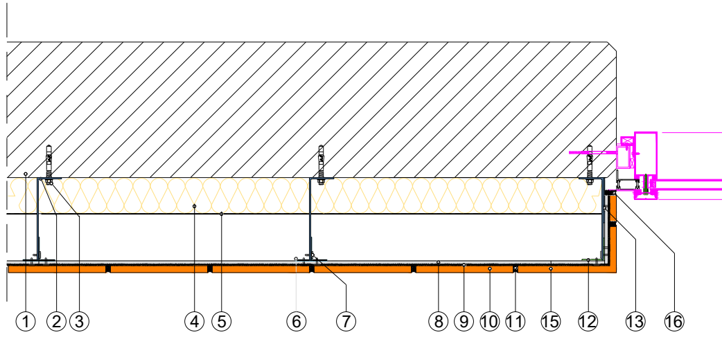
WINDOW EDGE CONNECTION PLAN
