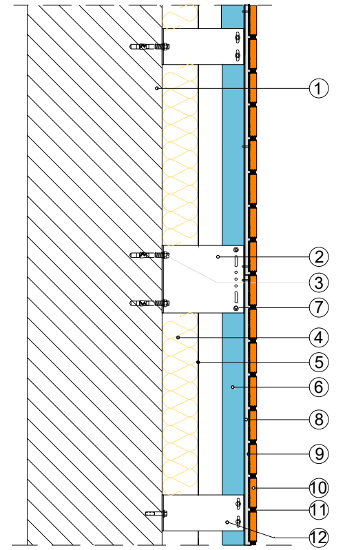
SECTION
